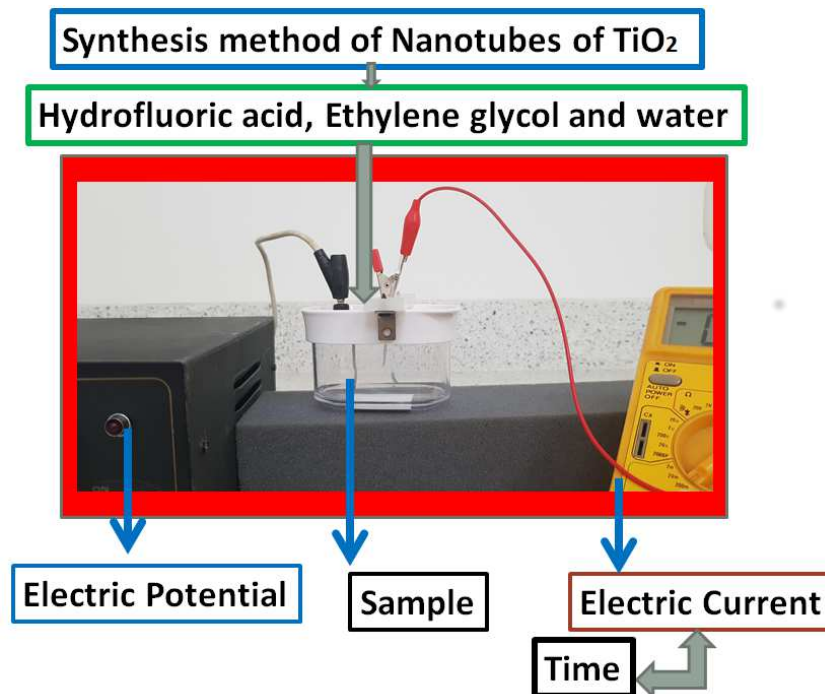
Figure 1. Experimental procedure for obtaining nanotubes from the titanium sheet.
