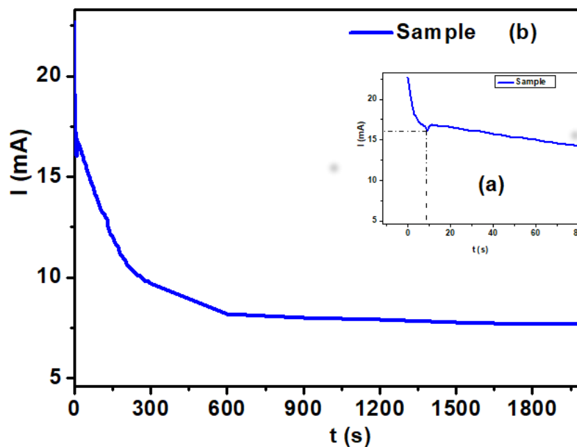
Figure 2. Electric current in (mA) as a function of the anodized time (s). For a sample subjected to 40 min in the electrolyte. Figure (a) inserted magnification of the discontinuity region in the graph.
